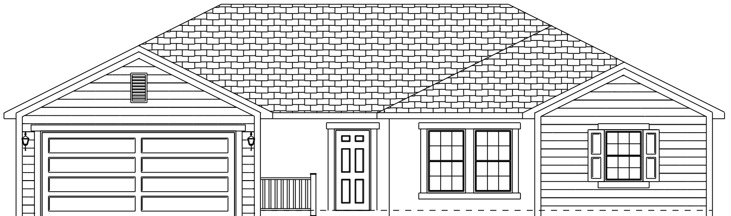
ELEVATION C
